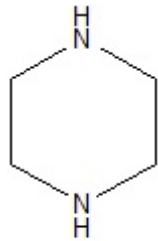
Piperazine
